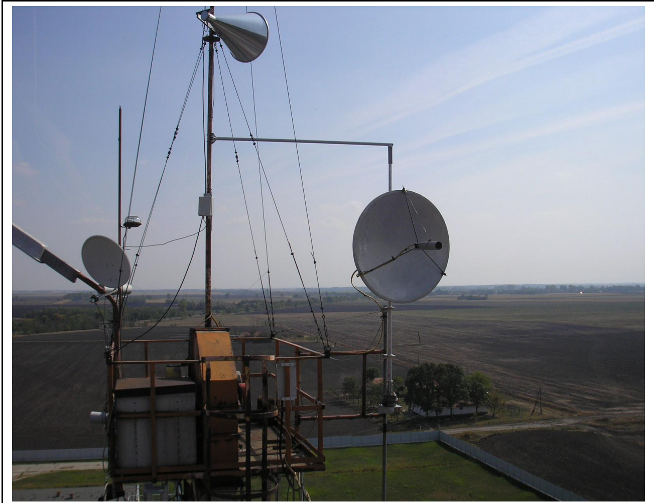
HA8MV dish-view
