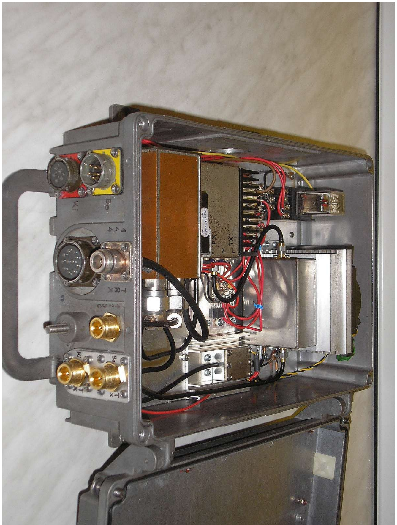
HA8MV's new portable 23cm TCRV
